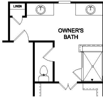
OPTIONAL OWNER'S BATH 1
